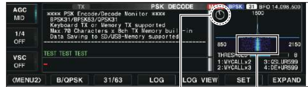
Vector tuning indicator Waterfall
