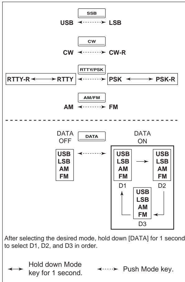
Mode keys
