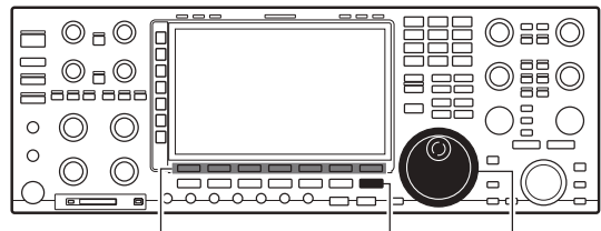
(F) Function keys [EXIT/SET] [MAIN DIAL]
