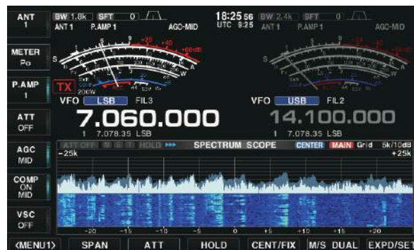
(F) Function keys [EXIT/SET] [MAIN DIAL]
