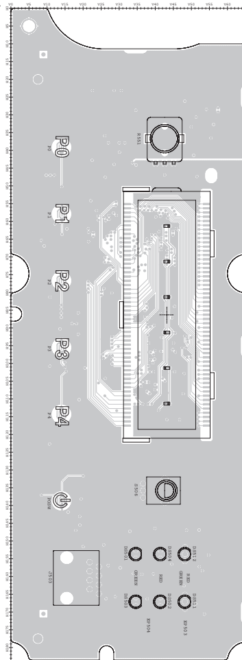
• FRONT UNIT (TOP VIEW)
