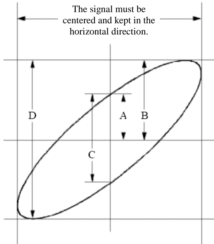
Figure 6-6 Lissajous Graph
