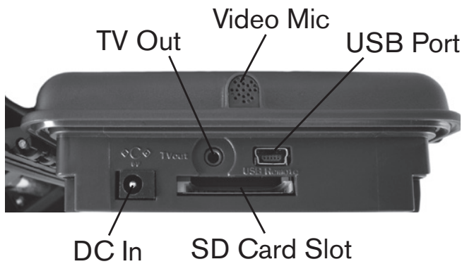
Fig. 1: Connections
