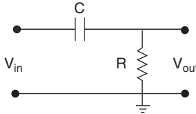
Figure 2-27. Simple RC Highpass Circuit
