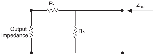
Figure 3-13. Electrical Circuit for Determining Output Impedance
