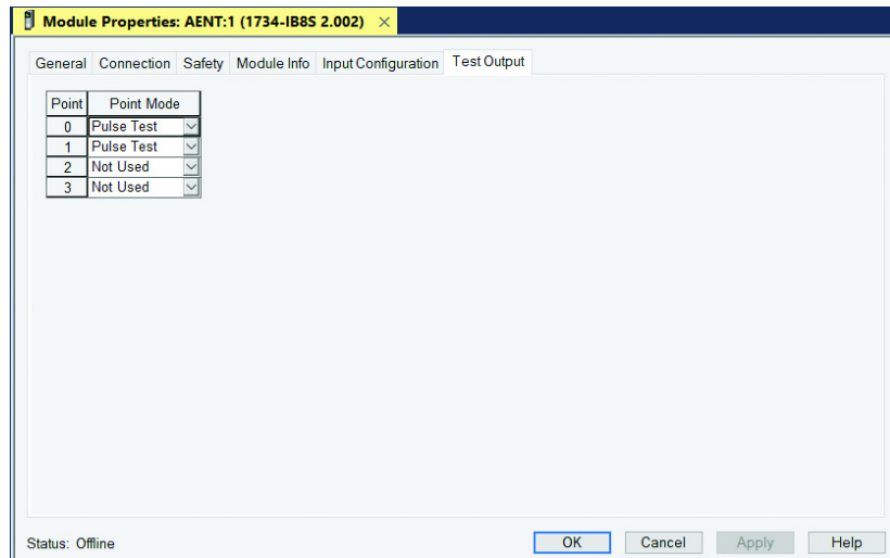
Figure 26 - 1734-IB8S Module Properties - Test Output
