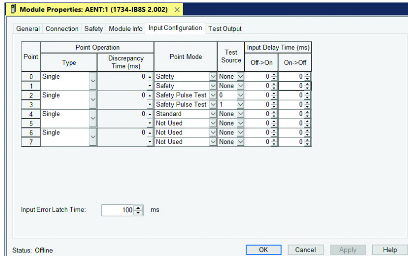
Figure 25 - 1734-IB8S Module Properties - Input Configuration
