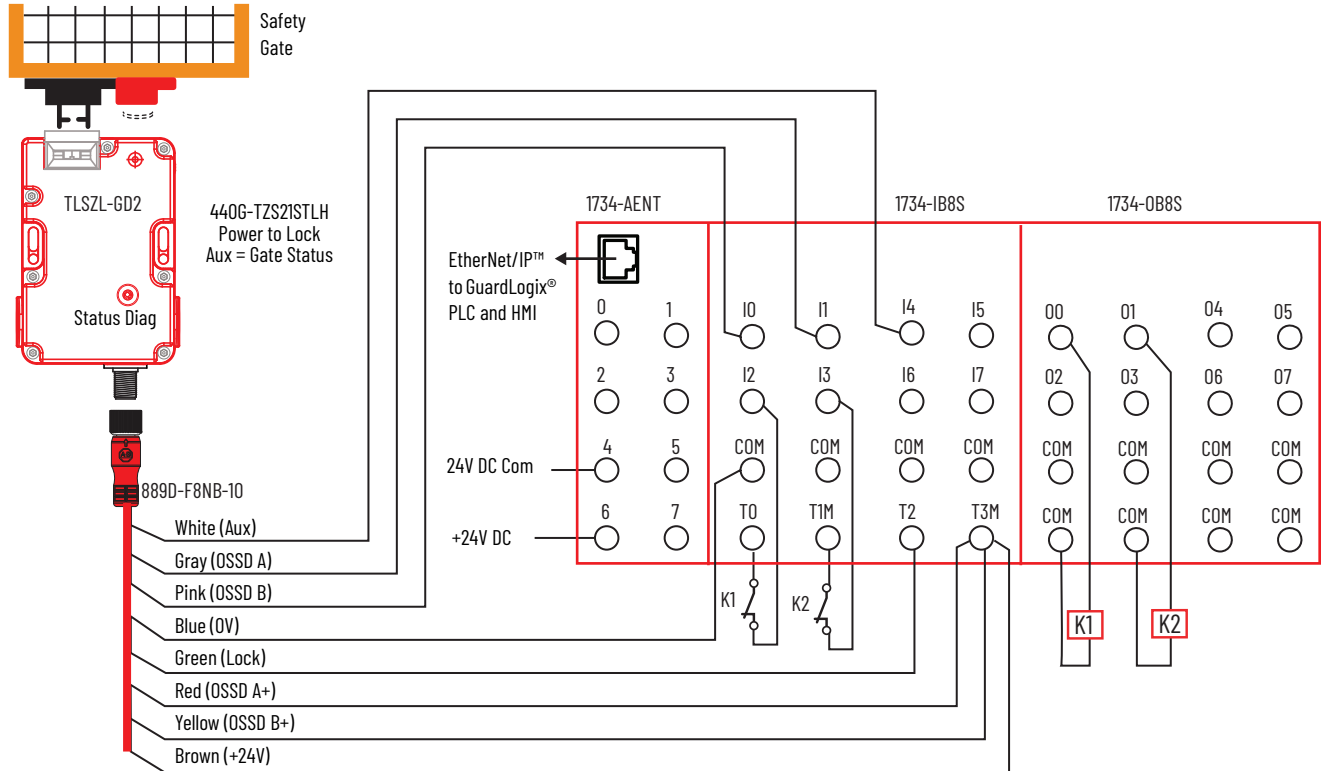
Figure 23 - 1734 and TLSZL Schematic
