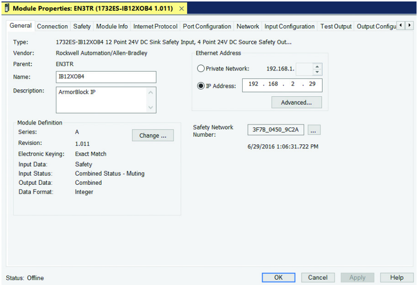
Figure 31 - Module Properties - General
