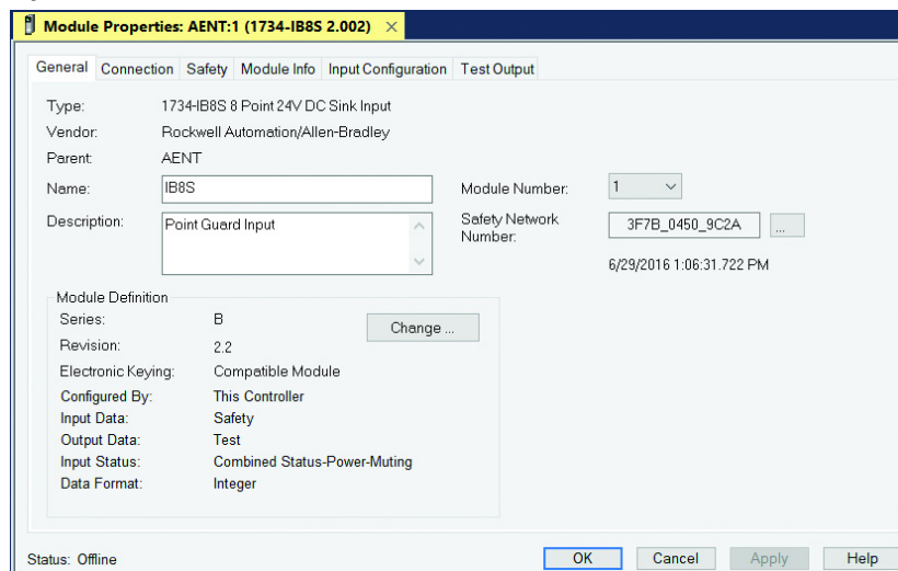
Figure 24 - 1734-IB8S Module Properties - General
