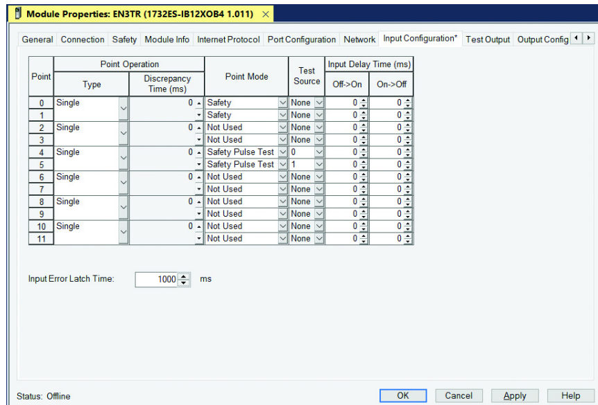
Figure 32 - Module Properties - Input Configuration
