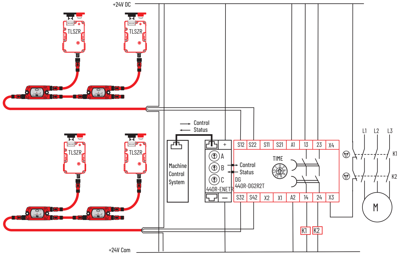
Figure 20 - DG with TLSZR Schematic
