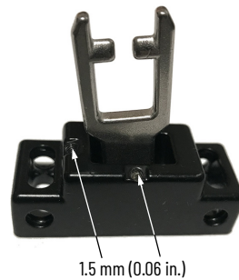
Figure 5 - Actuator Set Screw
