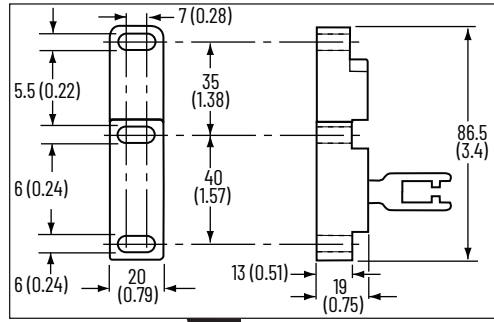
Figure 13 - Actuator/Target Mounting Dimensions [mm (in.)]
