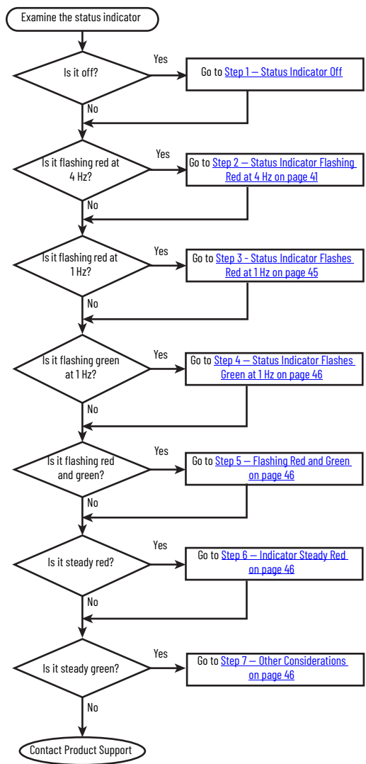
Figure 36 - Troubleshooting Flow Diagram
