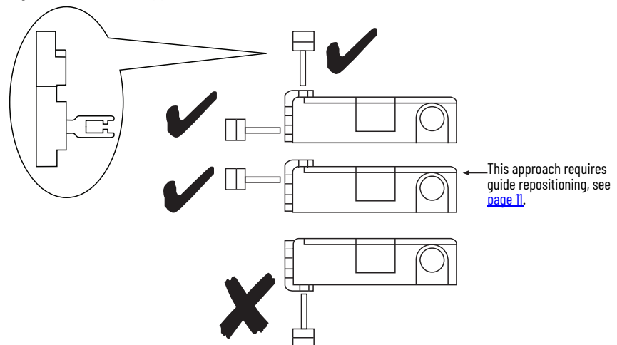
Figure 3 - Allowable Approach Direction
