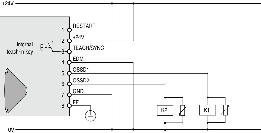
Figure 21 - Connecting the SC300 without external device monitoring (EDM), without internal restart interlock and without external key-operated pushbutton for teach-in
