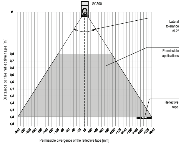
Figure 19 - Permissible divergence of the reflective tape from the optical axis of the camera as a function of the distance at 30 mm resolution (illustration of divergence not to scale)
