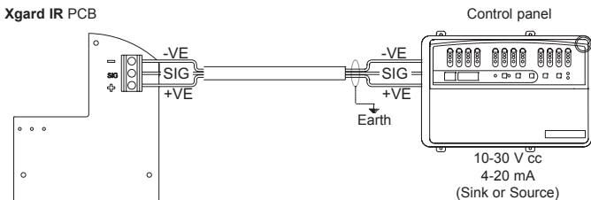
Diagram 5: Xgard IR electrical connections
