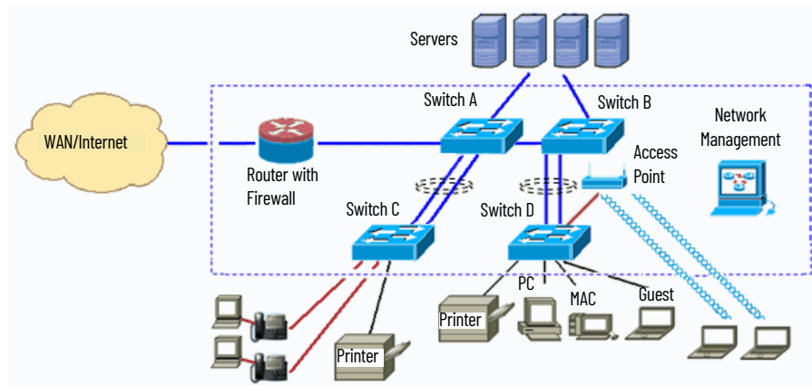
Figure 12 - EtherChannel Example
