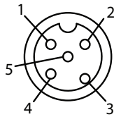
Figure 72 - Console Port Pinout
