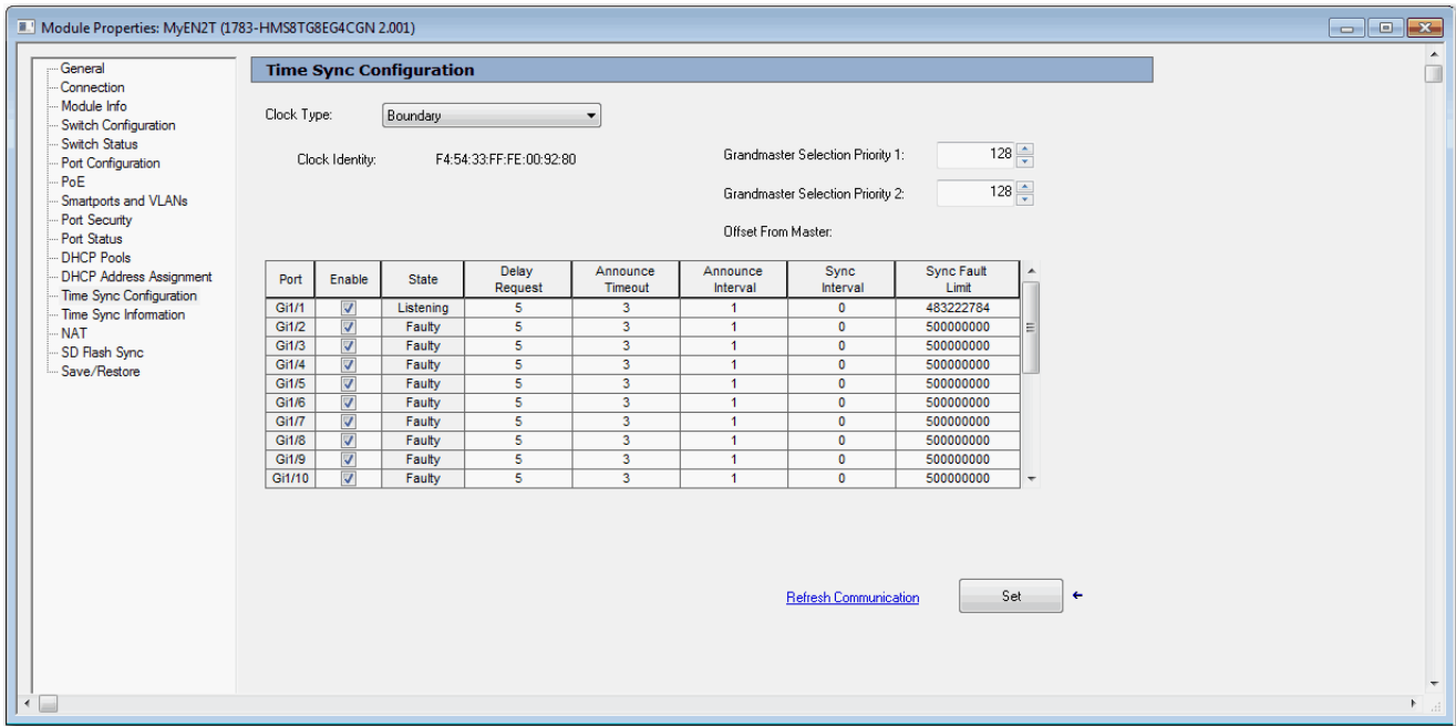
Figure 7 - Boundary Mode
