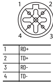
Figure 65 - 10/100 Connector Pinouts
