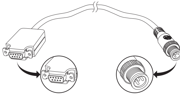
Figure 71 - M12-to-DB-9 Cable
