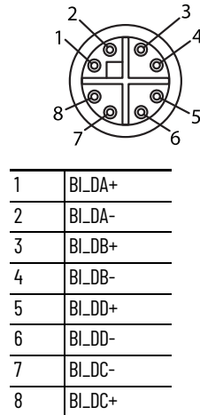
Figure 66 - 100/1000 Connector Pinouts
