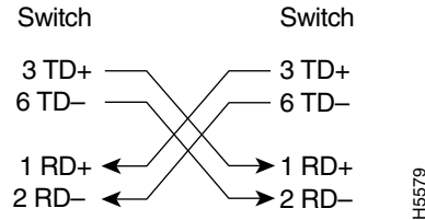
Figure 69 - Two Twisted-pair Crossover Cable Schematics
