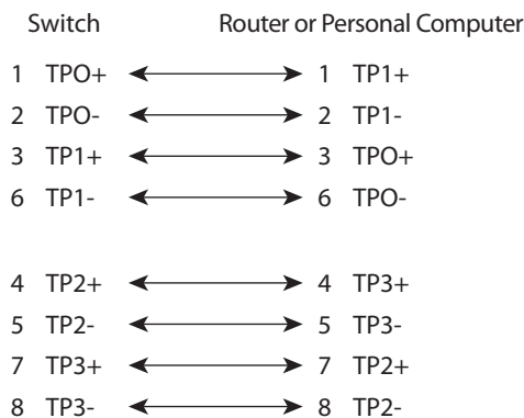
Figure 51 - Four Twisted-pair Straight-through Cable Schematics
