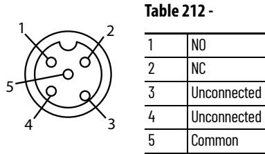
Figure 75 - Wiring Example for Alarm Inputs and Outputs
