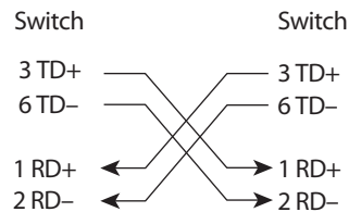
Figure 81 - Two Twisted-pair Crossover Cable Schematics
