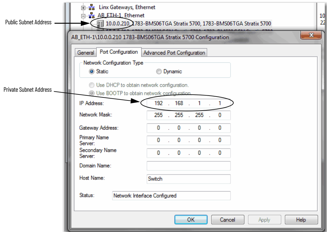
Figure 20 - Public and Private Subnet Addresses in Linux-based Software
