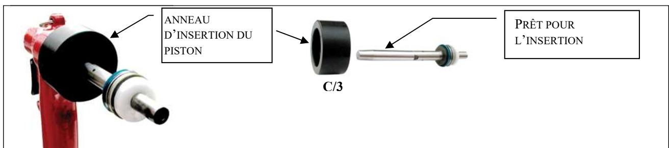
Figure 7.3 – D – Instructions de montage
