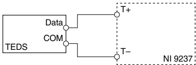
Figure 5. Connecting TEDS Sensors to the NI 9237
