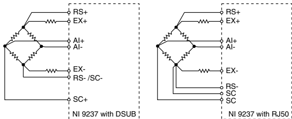
Figure 2. Connecting a Full Bridge to the NI 9237
