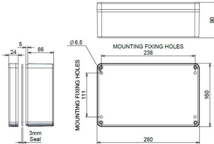
Figure 5 IMx-Rail enclosure drawing
