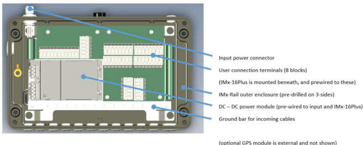
Figure 1 SKF Multilog IMx-Rail – arrangement of main system components
