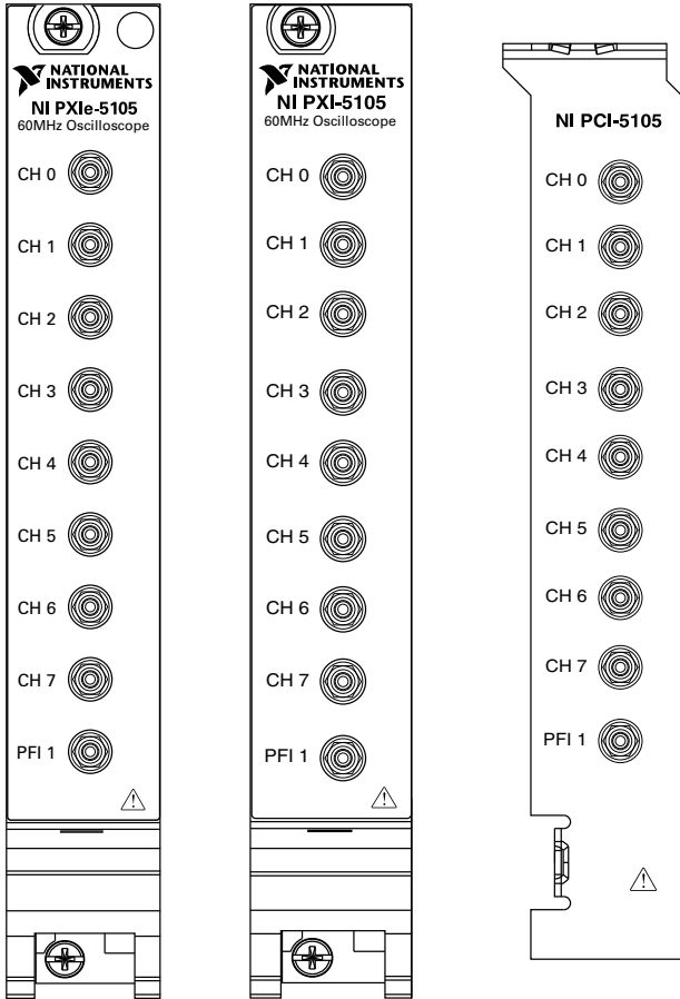
Figure 5. NI 5105 Front Panels
