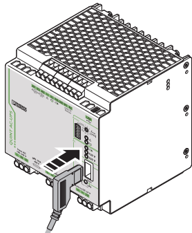
Figure 2 QUINT-UPS/1AC/1AC/500VA (Example)
