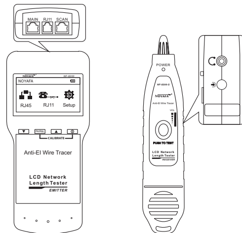
Main tester (NF-8200)
