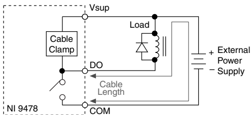
Figure 3. Cable Length of the NI 9478
