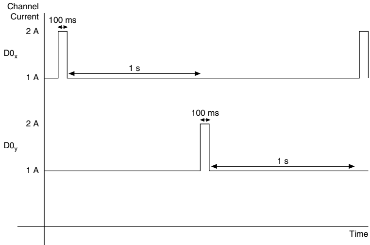
Figure 1. Short-circuit Behavior
