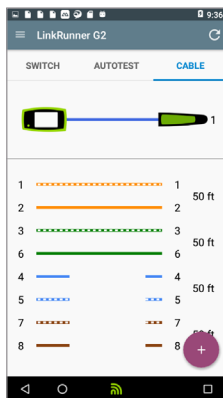
Wiremap Test
