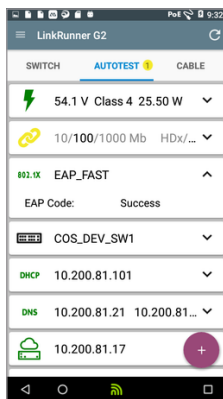
802.1x Results
