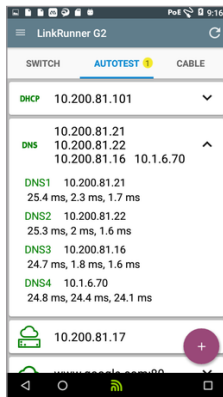
DNS Test
