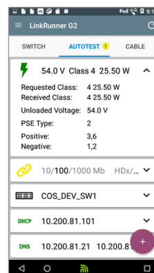
PoE Test
