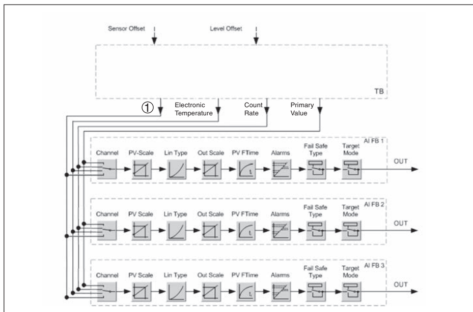
Рис. 28: FIBERTRAC 31: Block diagram with AI FB 1 ... AI FB 3 OUT values
