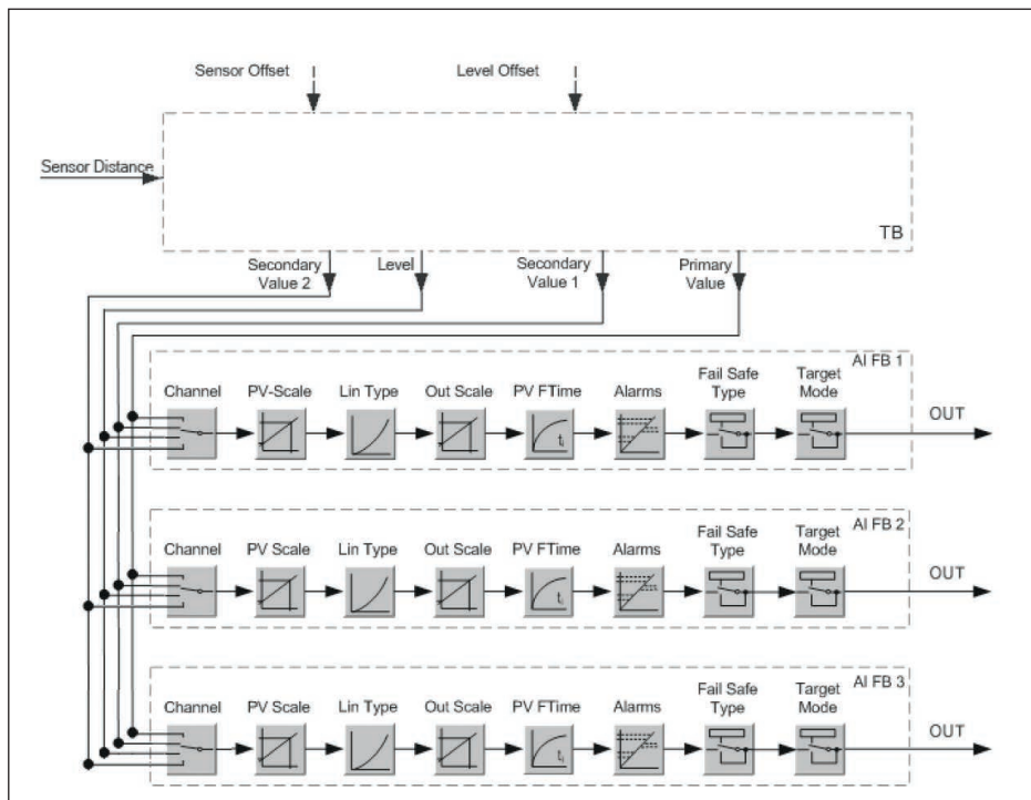
Рис. 47: VEGAPULS 65: Block diagram with AI FB 1 ... AI FB 3 OUT values
