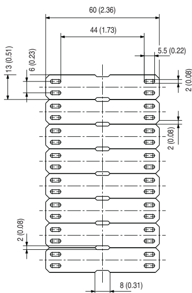
1492-MWCT11X60
